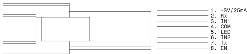
Fig.4: SPI terminals
